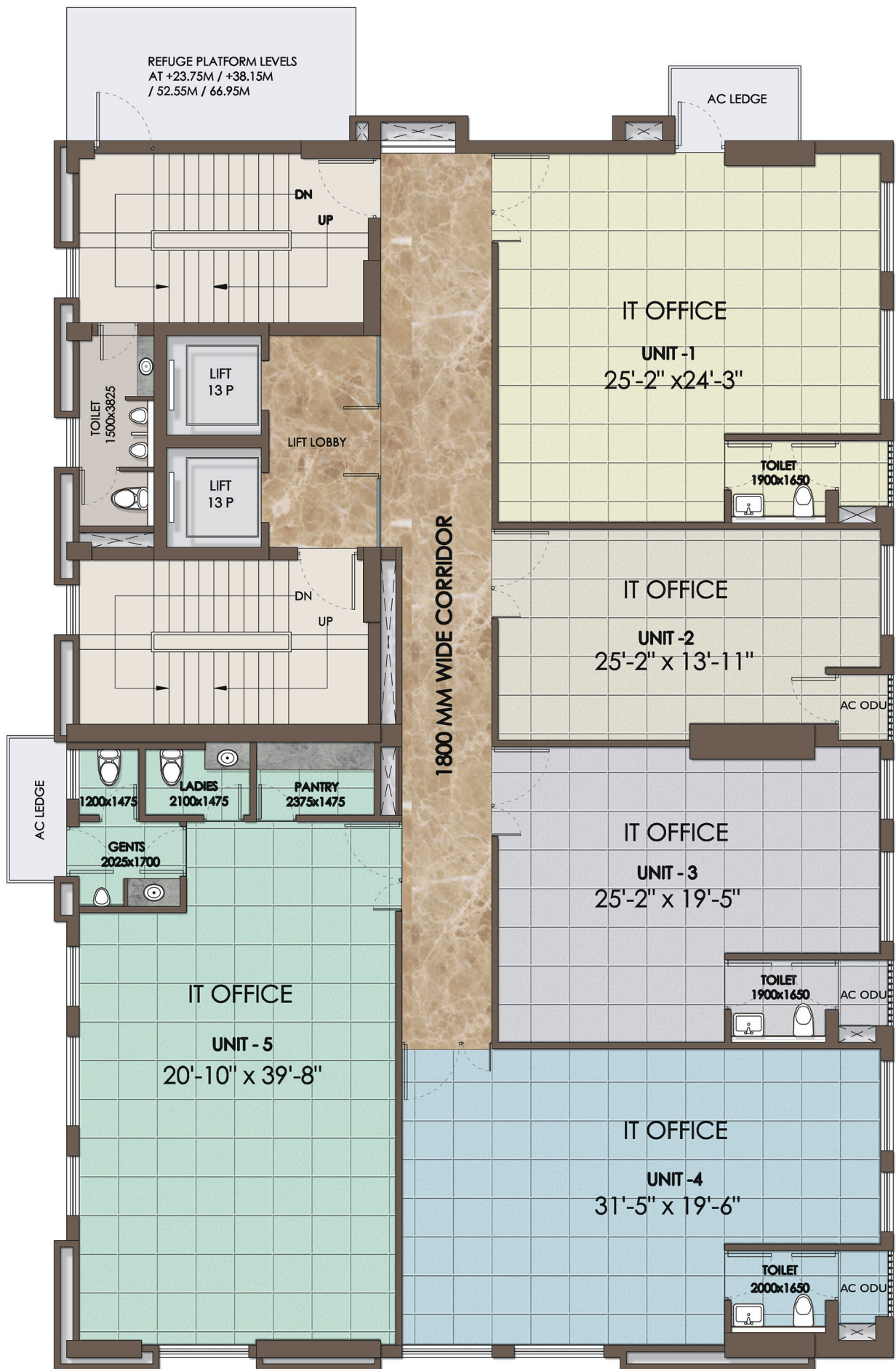
5TH-14TH FLOOR PLAN
